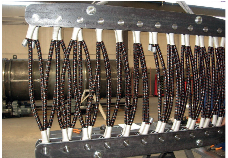
BILANCINO AD ELASTICI / BUNGEE LIFTING BEAM PORTATA / CAPACITY 12.500 Kg
