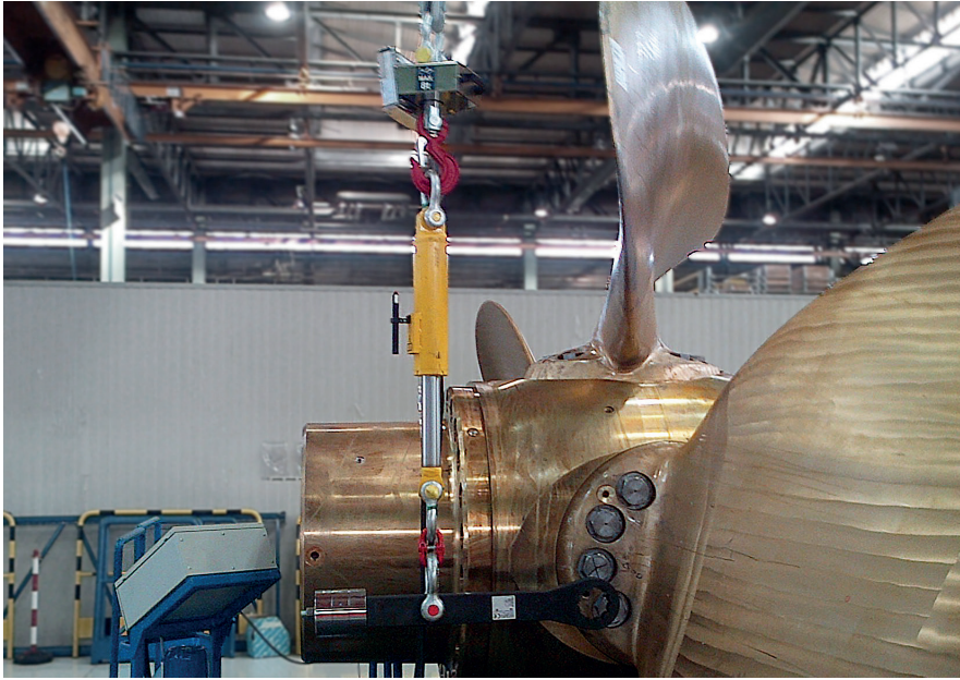
ATTREZZO SERRAGGIO DADI / EQUIPMENT FOR TIGHTENING NUTS PORTATA / CAPACITY 5.000 Kg
